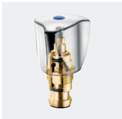
Water-free valve head with control knob
